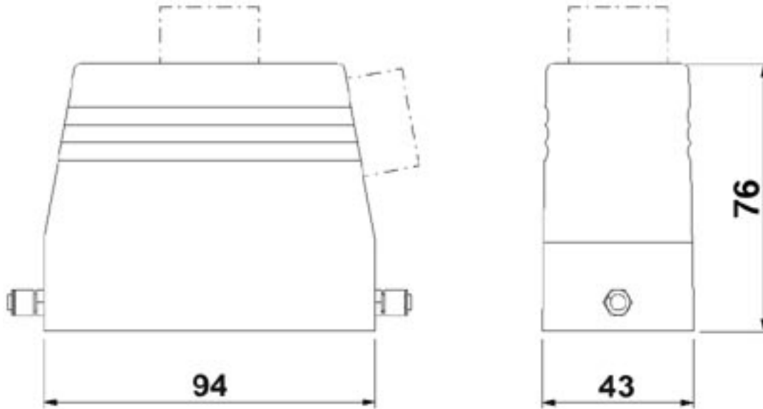
Dimensioned drawing
