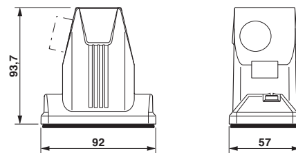
Dimensional drawing
