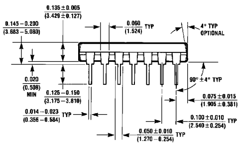
14-Lead Molded Dual-In-Line Package (N) Order Number DM74LS28N Package Number N14A
