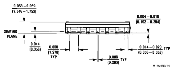
14-Lead Small Outline Molded Package (M) Order Number DM74LS28M Package Number M14A
