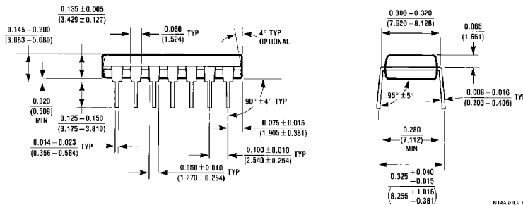
14-Lead Molded Dual-In-Line Package (N) Order Number DM74LS26N Package Number N14A
