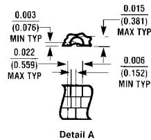
Ceramic Leadless Chip Carrier Package (E) Order Number 54LS09LMQB Package Number E20A
