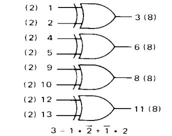
MC1812/MC1912 Quad 2-Input Exclusive OR Gate
