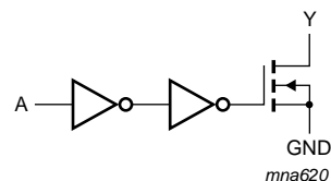
Fig 3. Logic diagram
