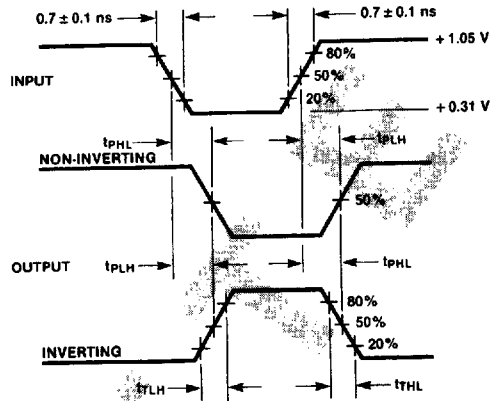
FIGURE 2. Output Rise and Fall Times and Waveforms
