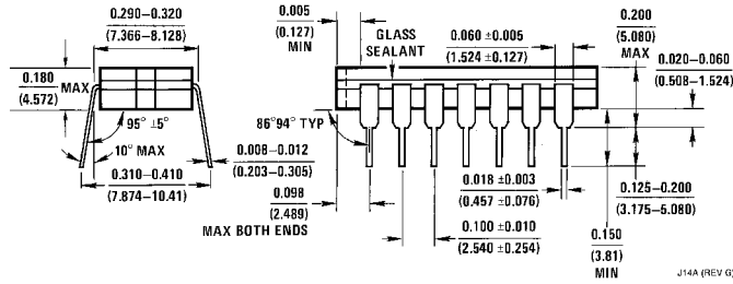
14-Lead Ceramic Dual-In-Line Package (J) Order Number DM5416J Package Number J14A
