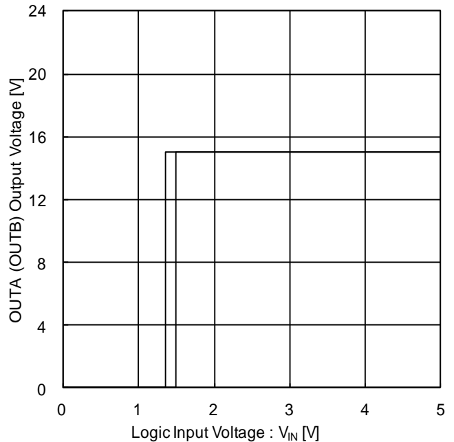
Figure 17. OUTA (OUTB) Output Voltage vs Logic Input Voltage (V CCB =15V, V CCA =15V, Ta=+25°C)
