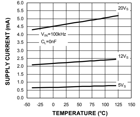
Supply Current (IS) vs. Temperature
