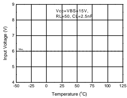
Figure 9a. Logic "0" IN Voltage vs Temperature
