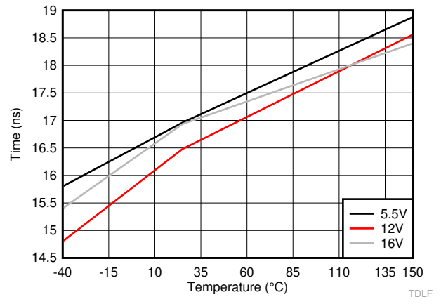
Figure 6-24. HO Falling Propagation Delay (TDHFF)
