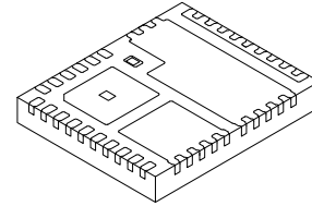
PQFN39 MN SUFFIX CASE 483BF
