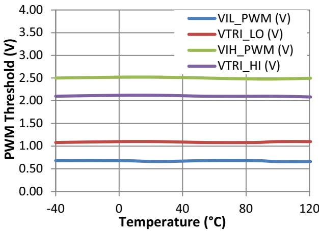
Figure 14. PWM Threshold vs. Temperature
