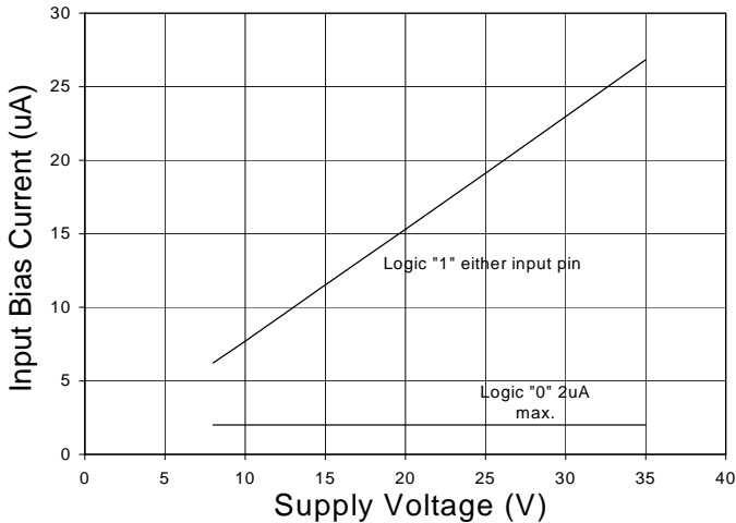
LIN / HIN Bias Current vs. Supply Voltage
