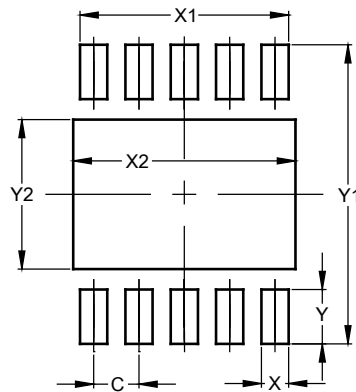
V-DFN3030-10 (Standard)
