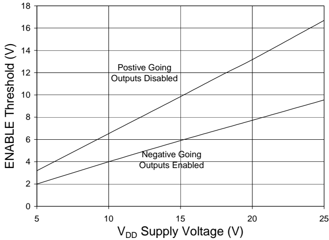
Enable Threshold vs. V_{DD} Logic Supply Voltage Active Low Enable
