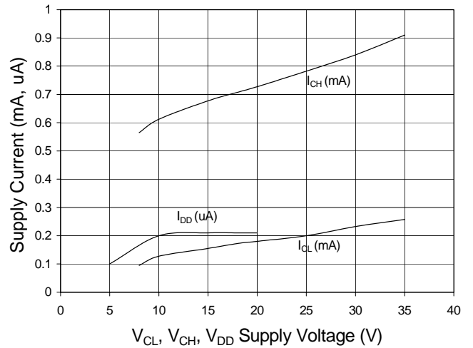
Quiescent Supply Currents vs. Supply Voltages V_{INL}, V_{INH} = 0V
