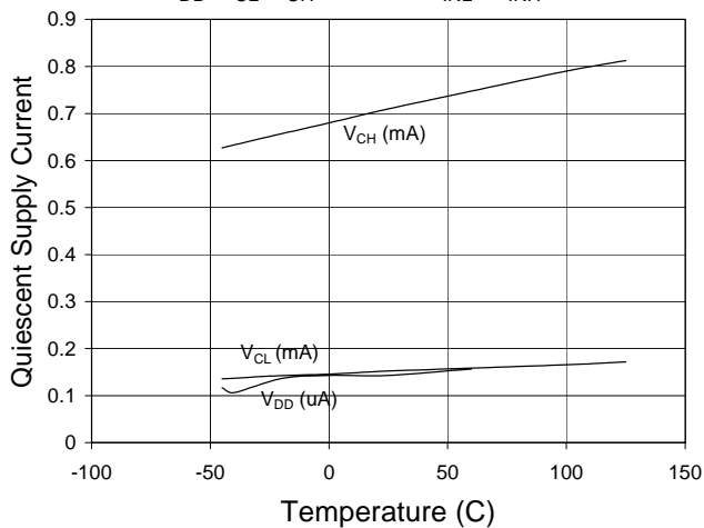
Quiescent Supply Current vs. Temperature V_{DD}, V_{CL}, V_{CH} = 15V \quad V_{INL}, V_{INH} = 0V
