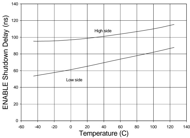
ENABLE Shutdown Delay vs. Temperature V_{DD}, V_{CL}, V_{CH} = 15V
