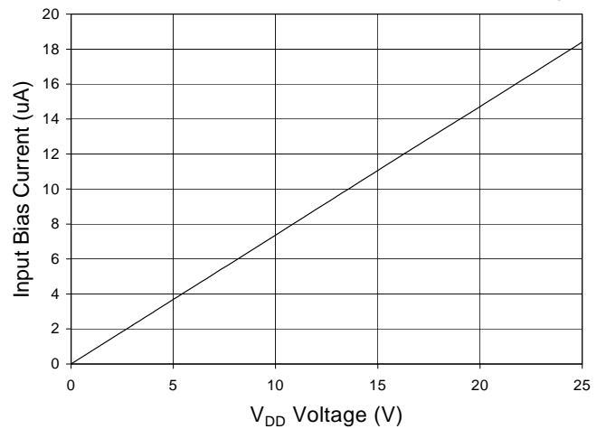
LIN, HIN Input Bias Current vs. V_{DD} Supply Voltage
