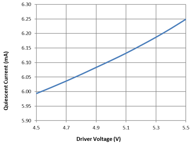
Figure 19. Quiescent Current vs. Driver Voltage
