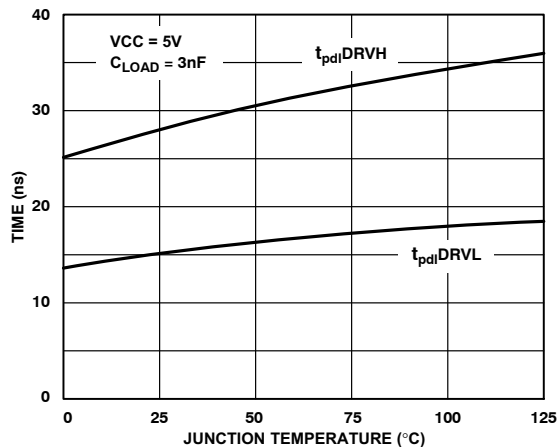
Figure 12. DRVH and DRVL t_{pdI} vs. Temperature
