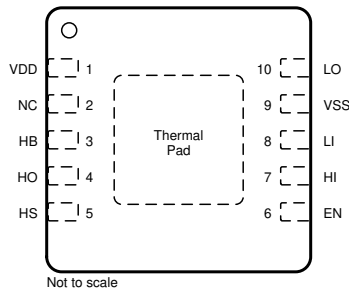
Figure 5-1. DRC Package 10-Pin VSON With Exposed Thermal Pad Top View
