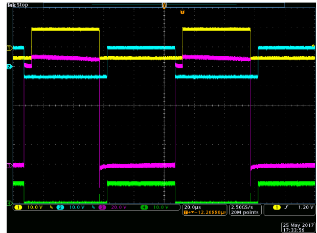
Figure 8-10. Input Negative Voltage
