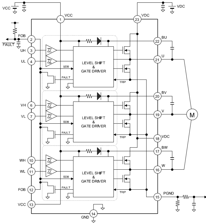
Figure 2. Block Diagram
