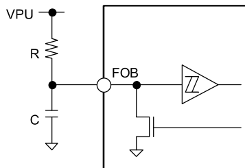
Figure 9. Release Time Setting Application Circuit
