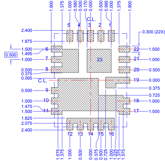
LAND PATTERN RECOMMENDATION SCALE 2:1
