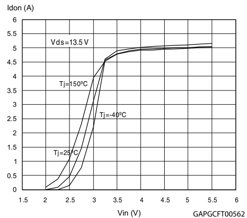
Figure 21. Transfer characteristics
