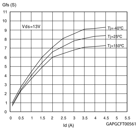
Figure 20. Transconductance
