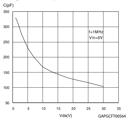
Figure 23. Capacitance variations
