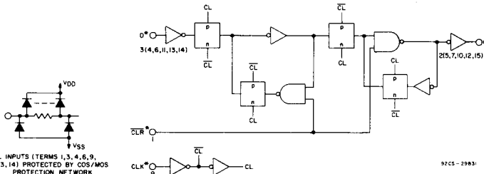
Fig. 1 - Logic diagram (1 of 6 flip-flops).
