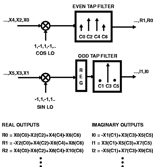
FIGURE 14. DOWN CONVERT AND DECIAMATE FUNCTION USING POLYPHASE FILTERS
