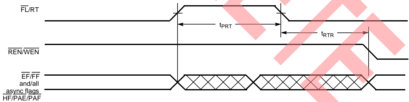
Figure 22. Retransmit Timing [33, 34, 35]
