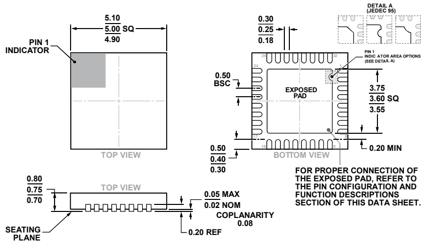
Figure 61. 32-Lead Lead Frame Chip Scale Package [LFCSPP] 5 mm x 5 mm Body and 0.75 mm Package Height (CP-32-12) Dimensions shown in millimeters
