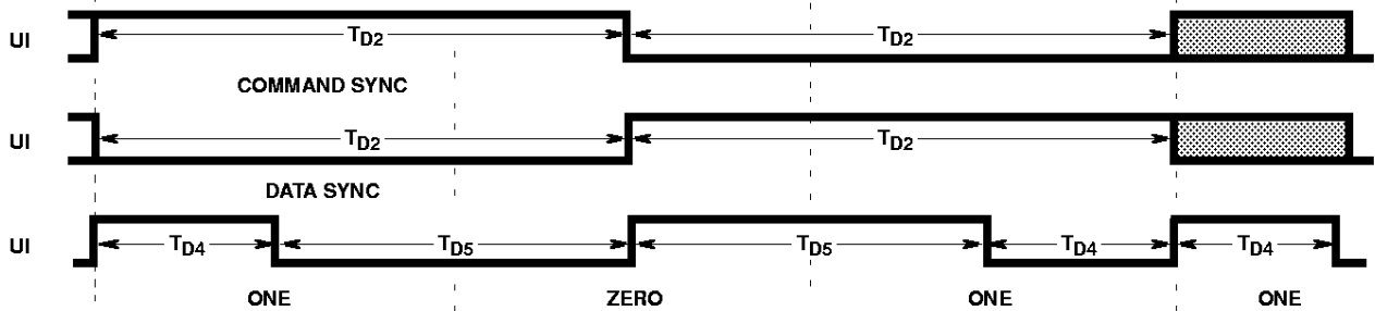
FIGURE 11. DECODER TIMING
