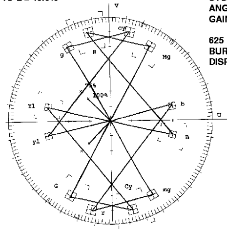
FIGURE 25. PAL COLOR BAR VECTOR SCAPE PLOT
