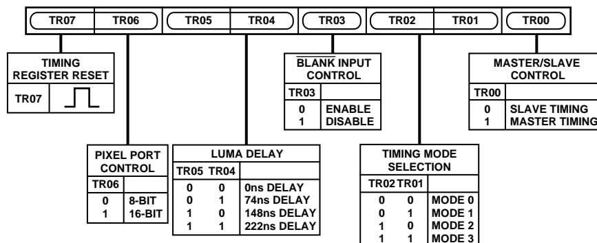
Figure 37. Timing Register 0
