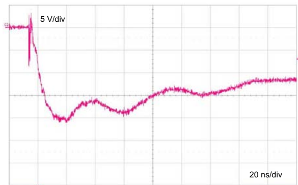
Figure 7. ESD response to ISO 10605- C = 330 pF, R = 330 \Omega (-15 kV contact)
