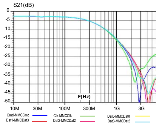
Figure 4. Attenuation versus frequency
