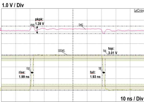
Figure 5. Digital crosstalk I6-O1
