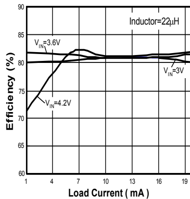
Main Display Efficiency ( 4LEDs )
