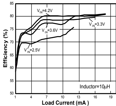
Sub Display Efficiency ( V_{SUB}=20V )
