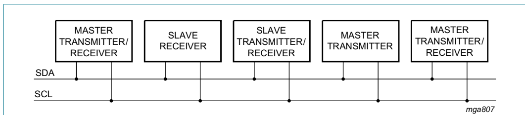
Fig 34. System configuration
