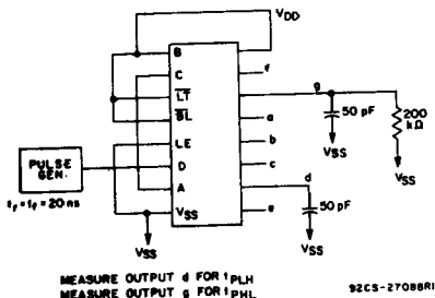
Fig. 12 - Data propagation delay.
