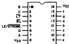
CD4511B TERMINAL ASSIGNMENT
