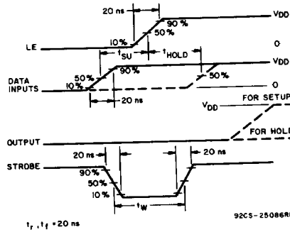
Fig. 14 - Dynamic waveforms.
