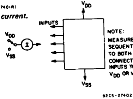
Fig. 11 - Input current.
