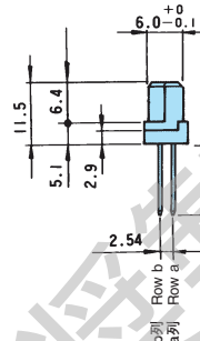
推奨取付寸法 Recommended mounting dimensions
