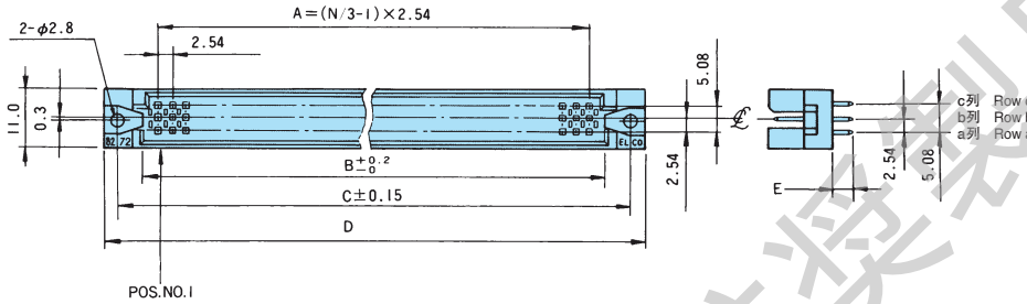
推奨取付寸法 Recommended mounting dimensions
