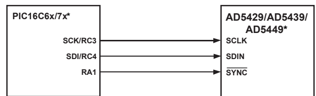
Figure 54. PIC16C6x/7x-to-AD5429/AD5439/AD5449 Interface
