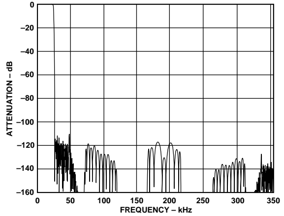
Figure 12. Complete Response, 8x Mode, 48 kHz Sample Rate
