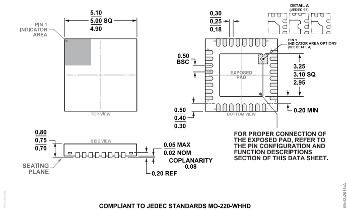
COMPLIANT TO JEDEC STANDARDS MO-220-WHHD Figure 91. 32-Lead Lead Frame Chip Scale Package [LFCSP] 5 mm x 5 mm and 0.75 mm Package Height (CP-32-7) Dimensions shown in millimeters
