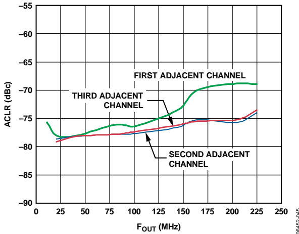
Figure 48. AD9776A ACLR vs. f_{OUT} , f_{DATA} = 122.88 \text{ MSPS} , 4x Interpolation, f_{DAC}/4 Modulation
