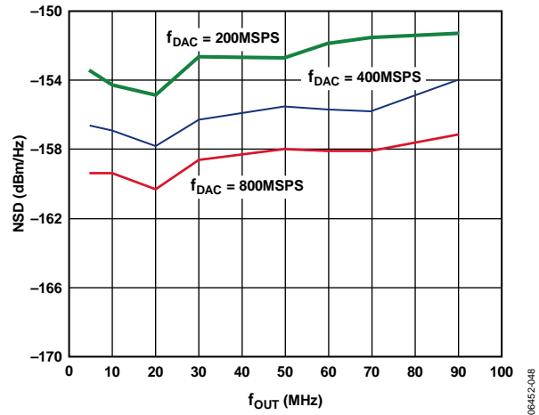
Figure 51. AD9776A Noise Spectral Density vs. f_{OUT} , Single-Tone Input at -6 dBFS, f_{DATA} = 200 \text{ MSPS}
