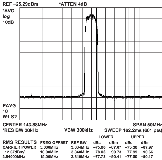
Figure 49. AD9776A Single Carrier W-CDMA, 4x Interpolation, f_{DATA} = 122.88 \text{ MSPS} , Amplitude = -3 dBFS
