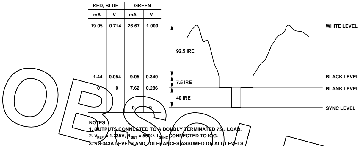
Figure 3. RGB Video Output Waveform
