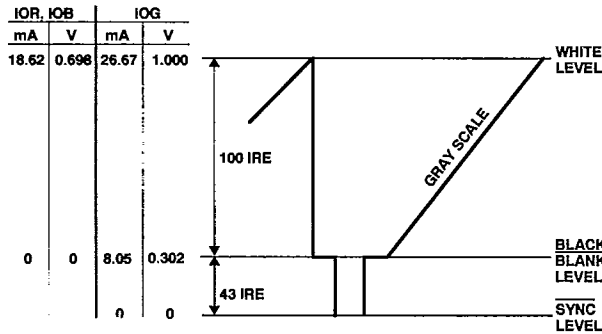
Figure 31. Composite Video Waveform SYNC Decoded on IOG; Pedestal = 0 IRE; R_{\text{SET}} = 265 \Omega
