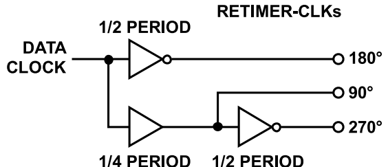
Figure 95. RETIMER-CLK Phases
