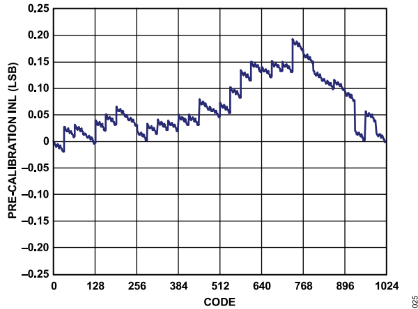
Figure 25. AD9115 Precalibration INL at 3.3 V, 20 mA
