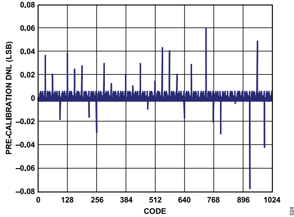
Figure 24. AD9115 Precalibration DNL at 1.8 V, 8 mA
