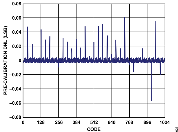
Figure 26. AD9115 Precalibration DNL at 3.3 V, 20 mA
