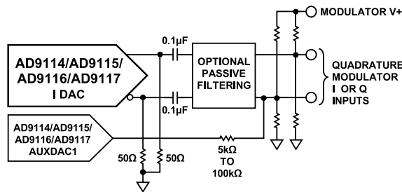
Figure 108. Typical Use of Auxiliary DACs
