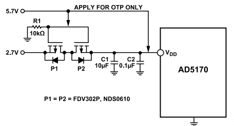
Figure 39. Isolate 5.7 V OTP Supply from 2.7 V Normal Operating Supply
