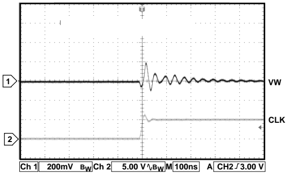
Figure 25. Digital Feedthrough
