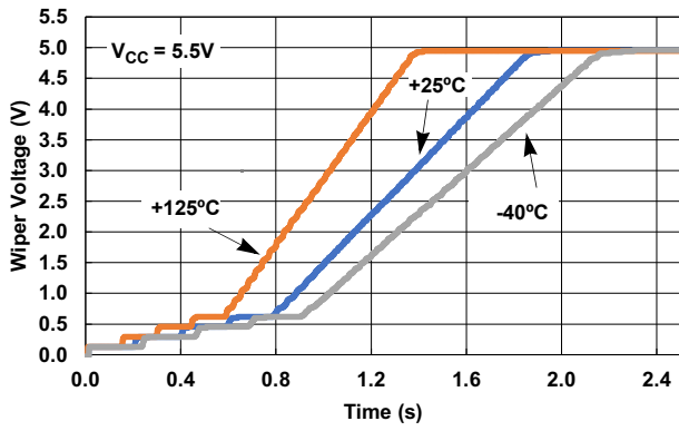
Figure 14. \overline{\text{PU}} Continuously Held Low, Fast Mode Timing (n = 9)
