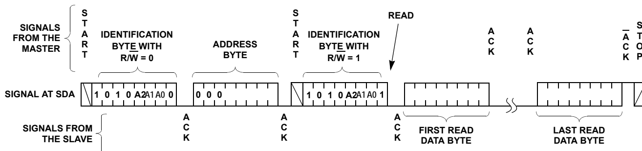
FIGURE 30. READ SEQUENCE
