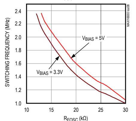
SWITCHING FREQUENCY vs. R FOSC (MAX16930)
