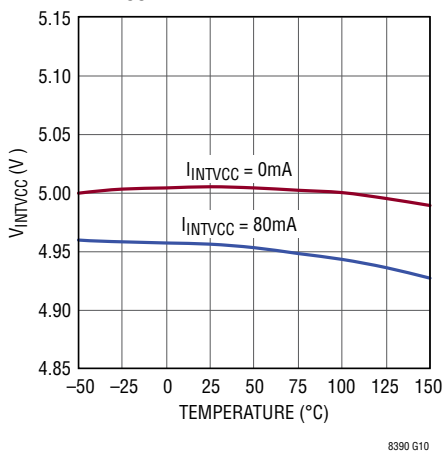
V_{INTVCC} Voltage vs Temperature
